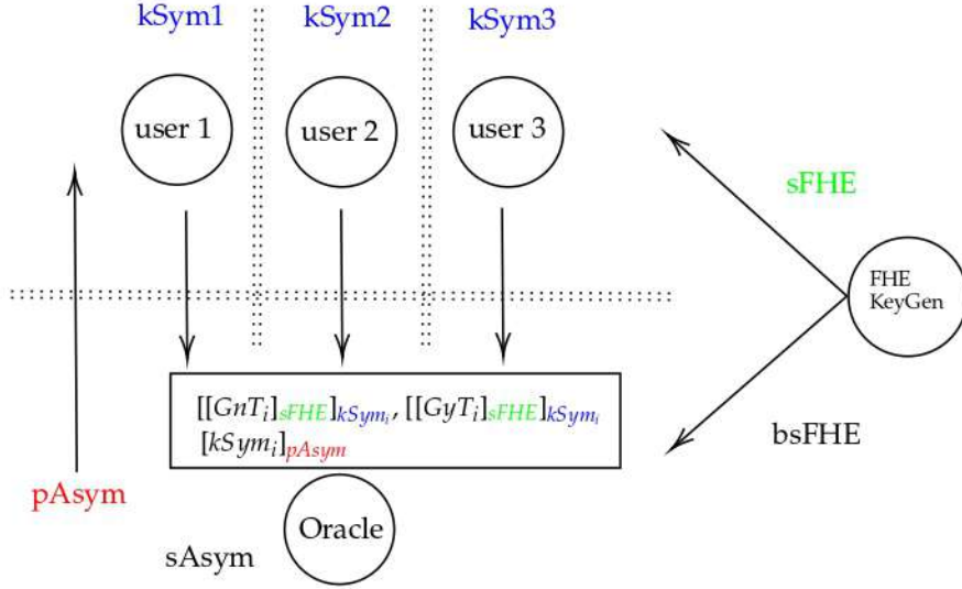
Fig. 5 Encrypted tokens
