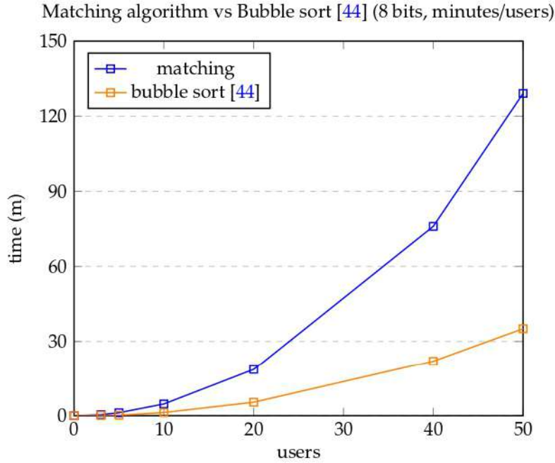
Fig. 10 Matching algorithm vs Bubble sort [44] graph
