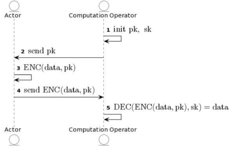
Fig. 1 Asymmetric encryption
